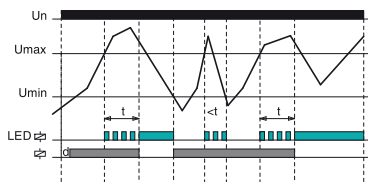
O2 OVER (hysteresis to Umin)
