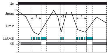
U1 UNDER (hysteresis 5%)
