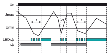
U2 UNDER (hysteresis to Umax)
