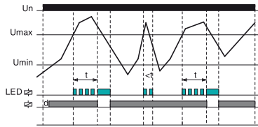
O1 OVER (hysteresis 5%)
