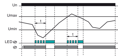
W WINDOW (hysteresis 5%)
