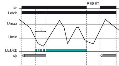
UL UNDER + Latch
