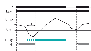
WL WINDOW + Latch
